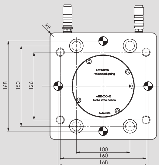
VIEW B
