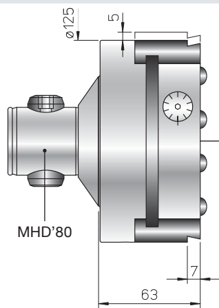
TRM 80/125 \varnothing 36-500
